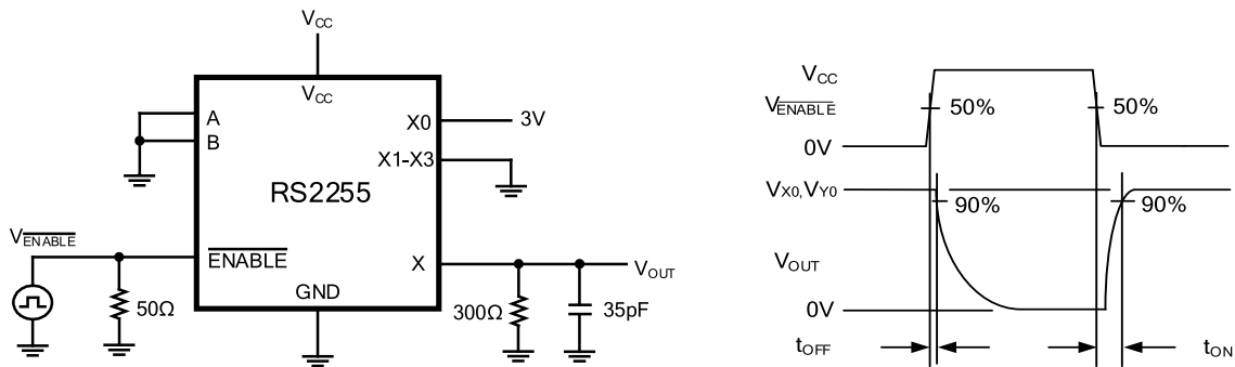
Test Circuit 2. Switching Times ( t_{\text{ON}} , t_{\text{OFF}} )
